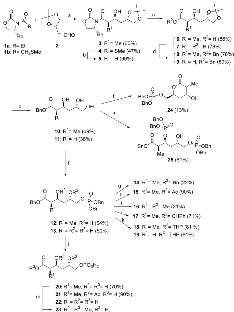
Scheme 1. (a) Bu 2 BOTf, CH 2 Cl 2 , Et 3 N, 0°C, then 2 , -78°C; (b) Bu 3 SnH, 1,1'-azobis(cyclohexanecarbonitrile), benzene, reflux, 2 h; (c) LiOH, H 2 O 2 , 0°C; (d) BnBr, K 2 CO 3 , DMF, rt; (e) CuCl 2 ·2H 2 O, i PrOH; (f) (BnO) 3 P, I 2 , -78°C, CH 2 Cl 2 ; (g) CCl 3 NHOBn, TfOH, CH 2 Cl 2 , rt; (h) Ac 2 O, DMAP, pyridine, rt; (i) MeO 3 BF 4 , DTBMP, CH 2 Cl 2 , rt; (j) PhCH(OMe) 2 , PPTS, DMF; (k) DHP, PPTS, CH 2 Cl 2 ; (l) H 2 , Pd/C, MeOH then HCl 1 M; (m) MeOH/HCl, rt.
